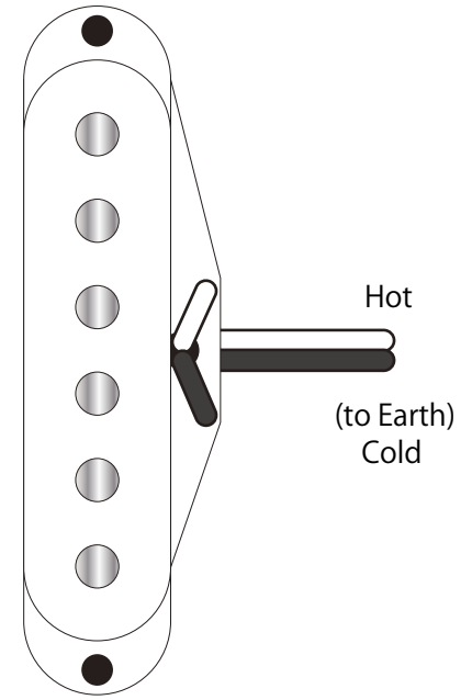
Bridge Pickup (North Top)
