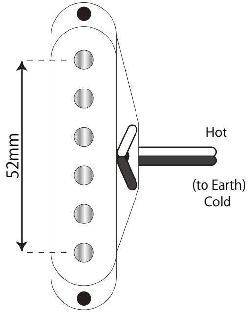
Neck Pickup (North Top)
