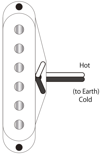
Middle Pickup (North Top)
